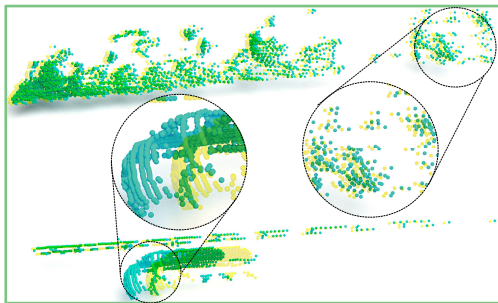
Ground Truth
