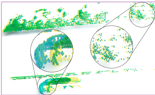
Our Method
