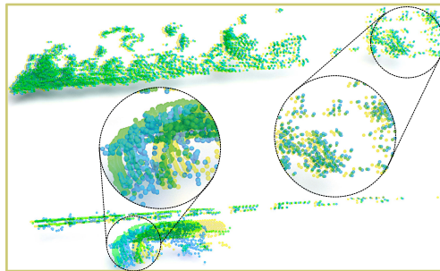
FLOT
