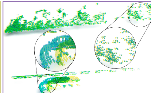
MSBRN
